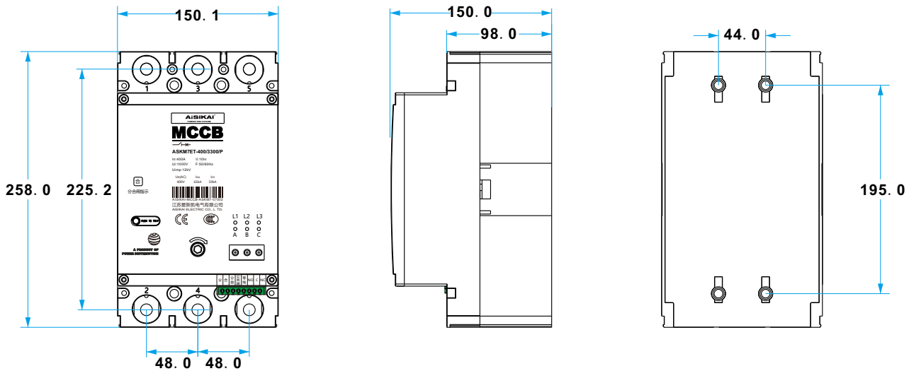
ASKM7ET-400A壳架
